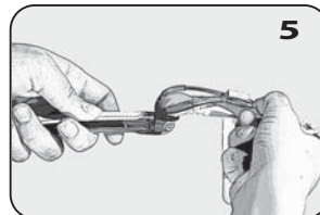
5 Place in Head
